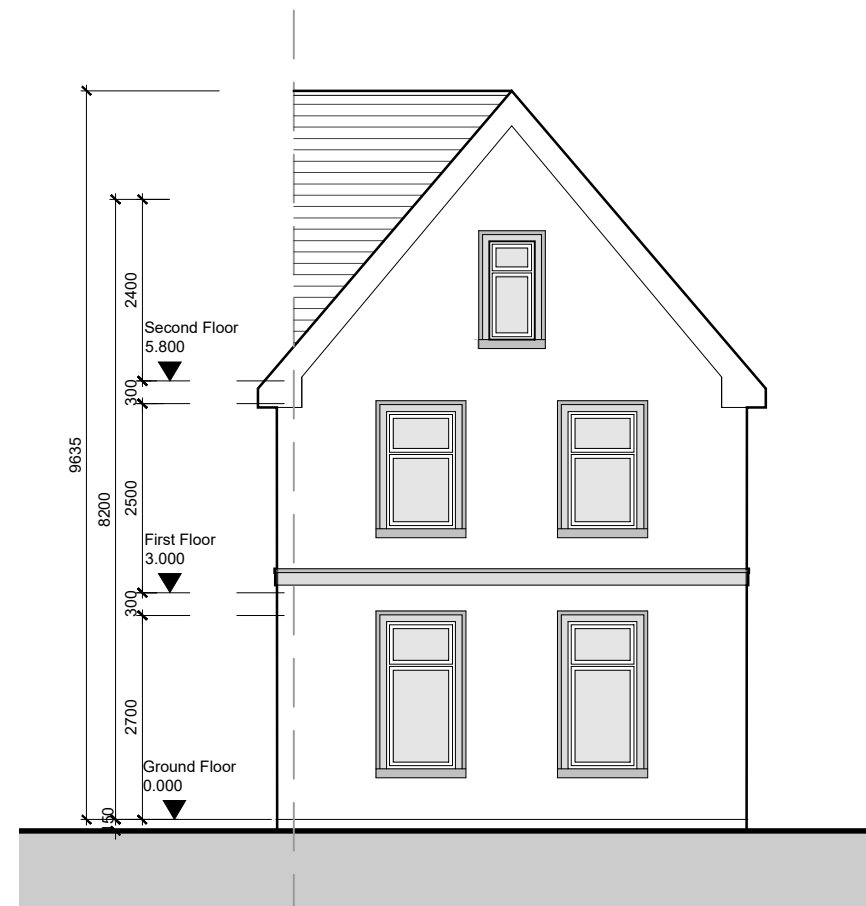
Side Elevation 01
