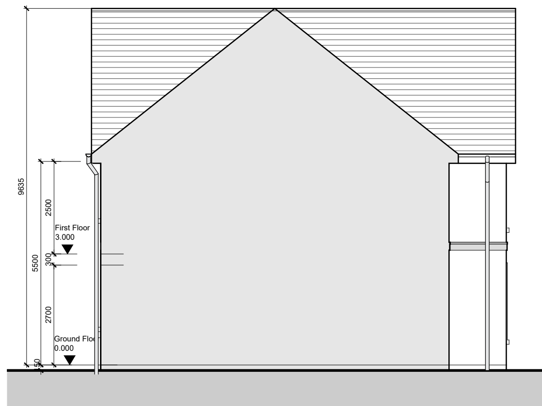
Side Elevation
